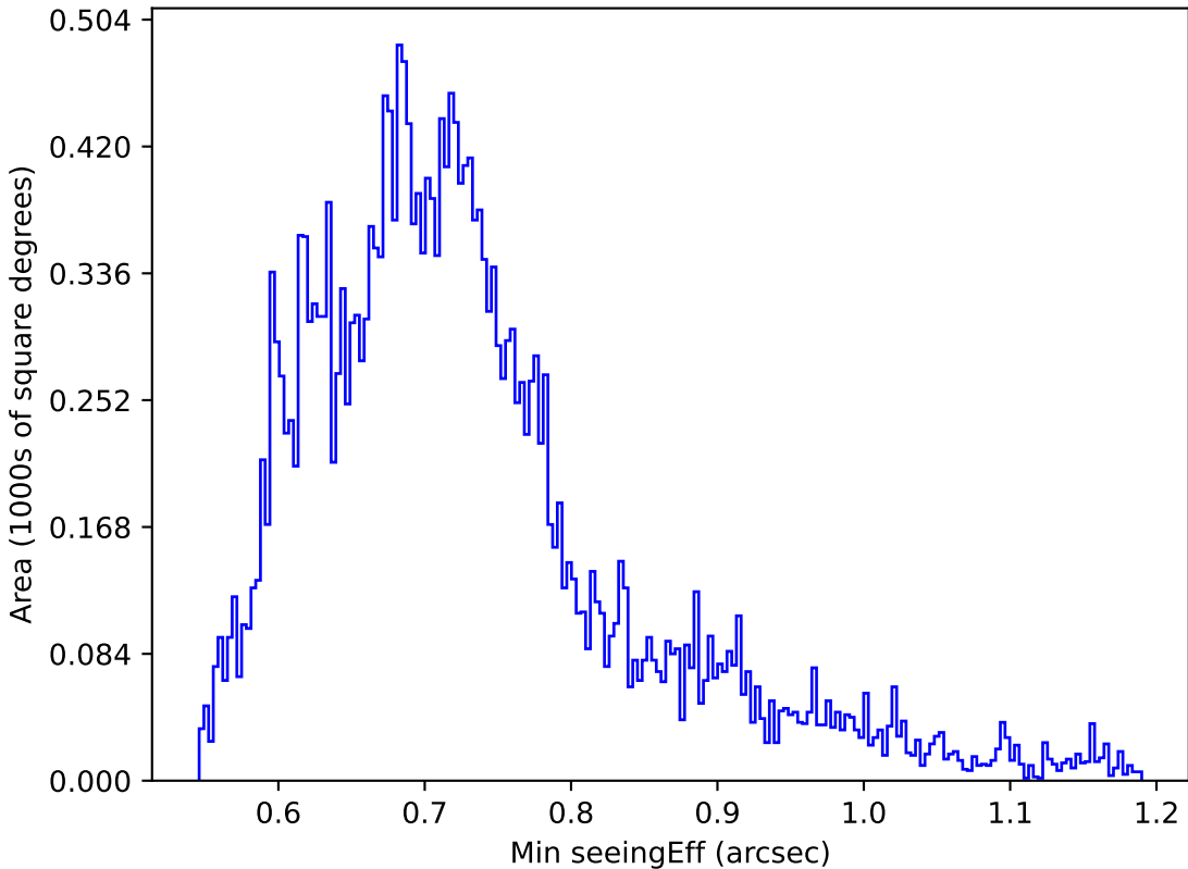
baseline_v2.0_10yrs Yr 1 r band: Min seeingEff
