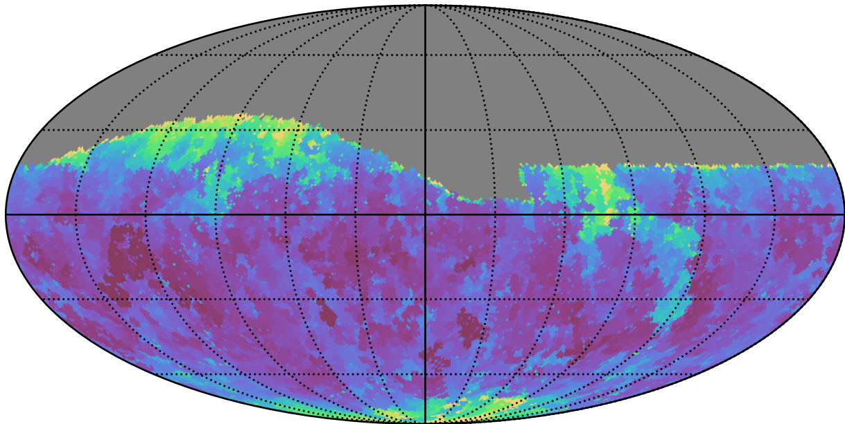
baseline_v2.0_10yrs Yr 1 i band: Min seeingEff
