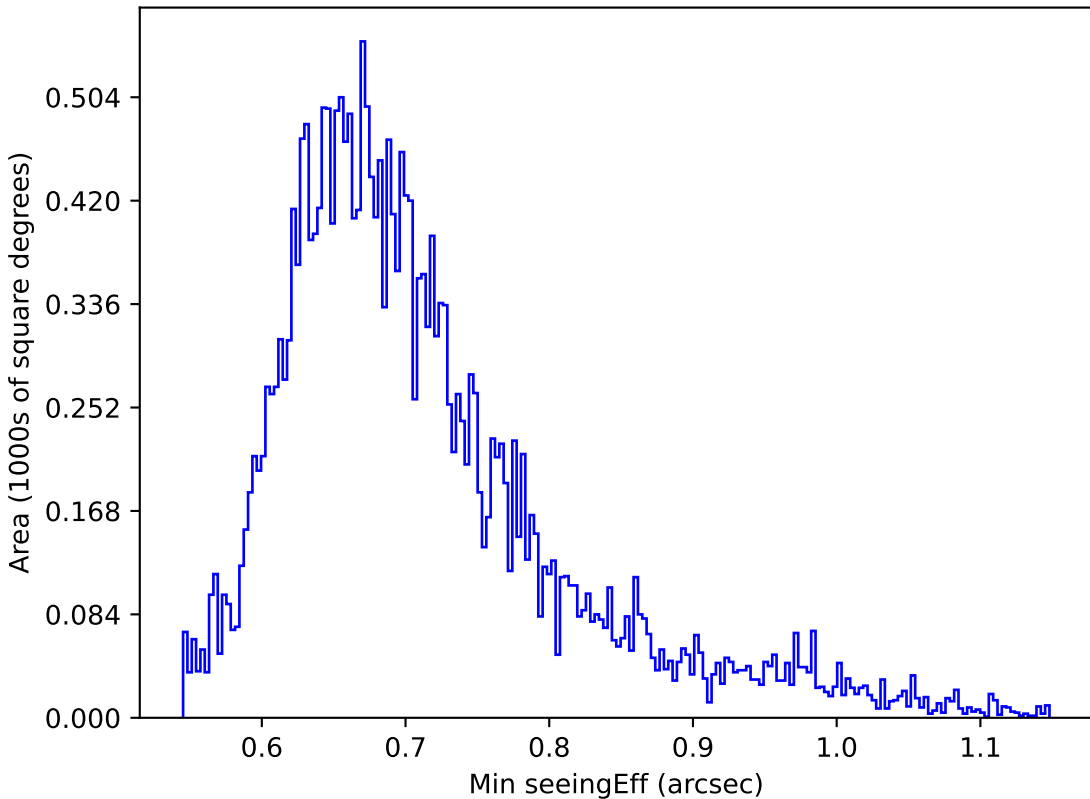
baseline_v2.0_10yrs Yr 1 i band: Min seeingEff
