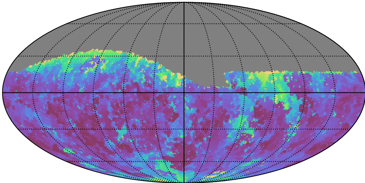
baseline_v2.0_10yrs Yr 1 g band: Min seeingEff
