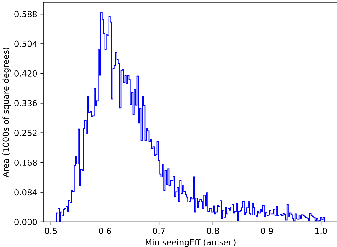
baseline_v2.0_10yrs Yr 1 all bands: Min seeingEff
