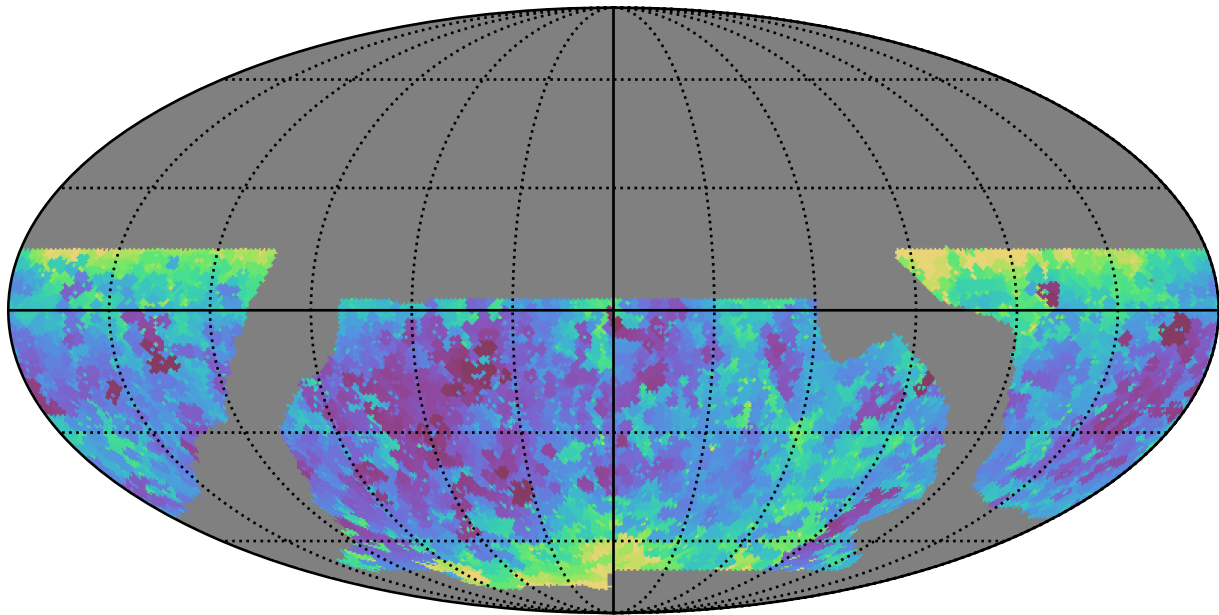
baseline_v2.0_10yrs WFD z band: Min seeingEff
