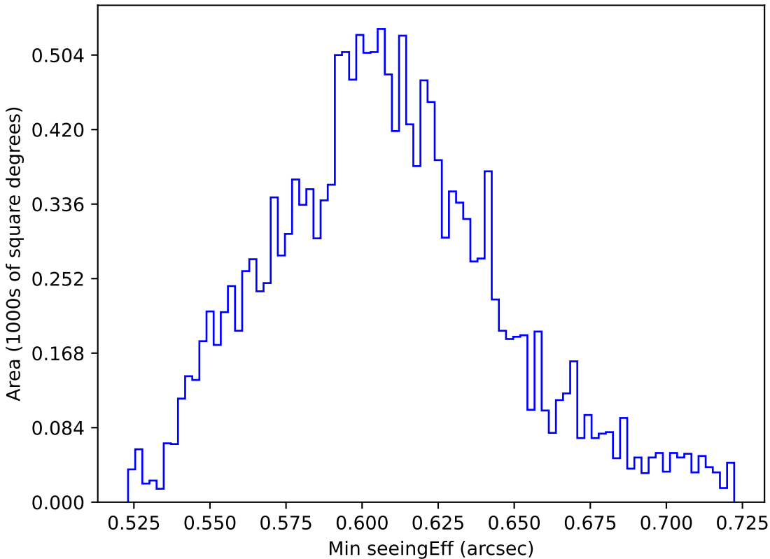
baseline_v2.0_10yrs WFD z band: Min seeingEff
