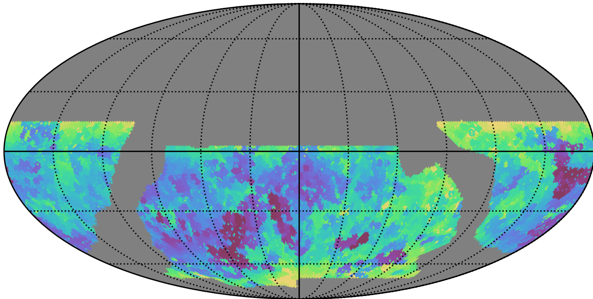
baseline_v2.0_10yrs WFD y band: Min seeingEff
