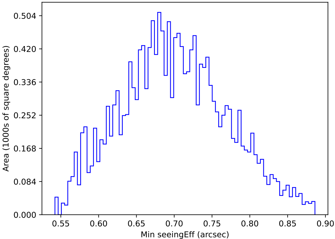
baseline_v2.0_10yrs WFD u band: Min seeingEff
