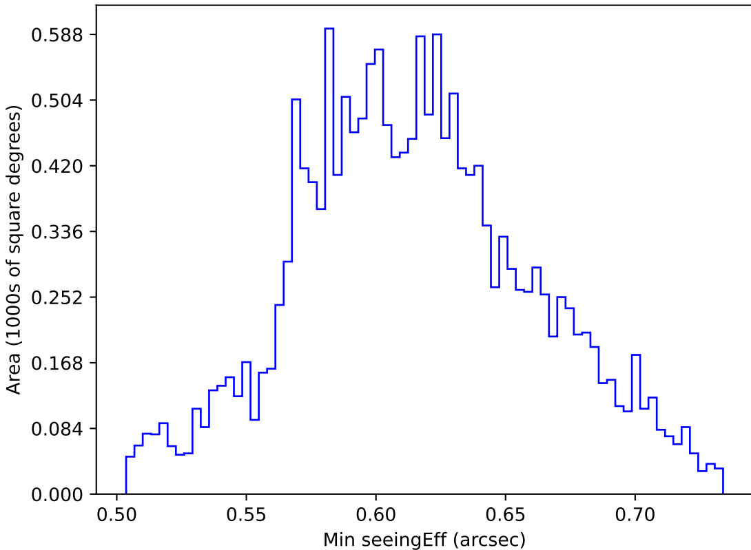
baseline_v2.0_10yrs WFD r band: Min seeingEff
