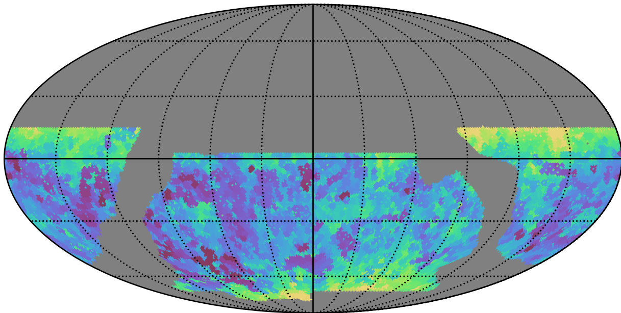
baseline_v2.0_10yrs WFD i band: Min seeingEff
