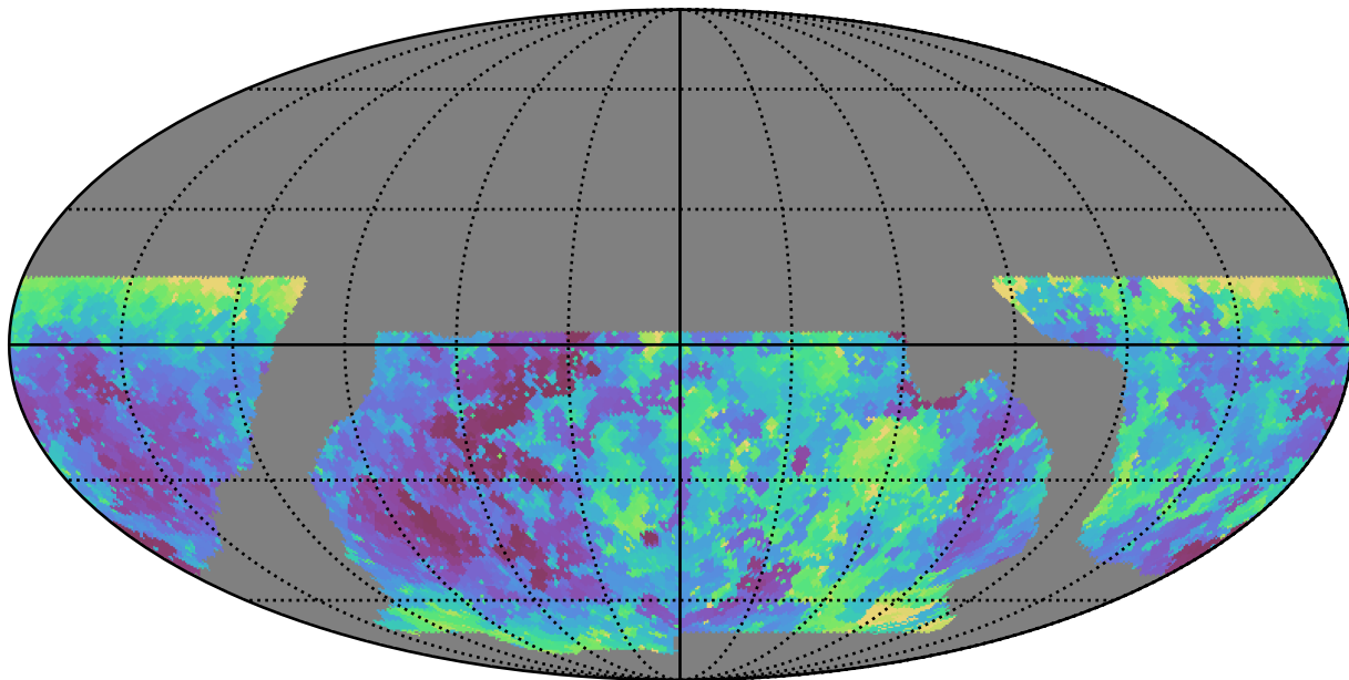
baseline_v2.0_10yrs WFD g band: Min seeingEff
