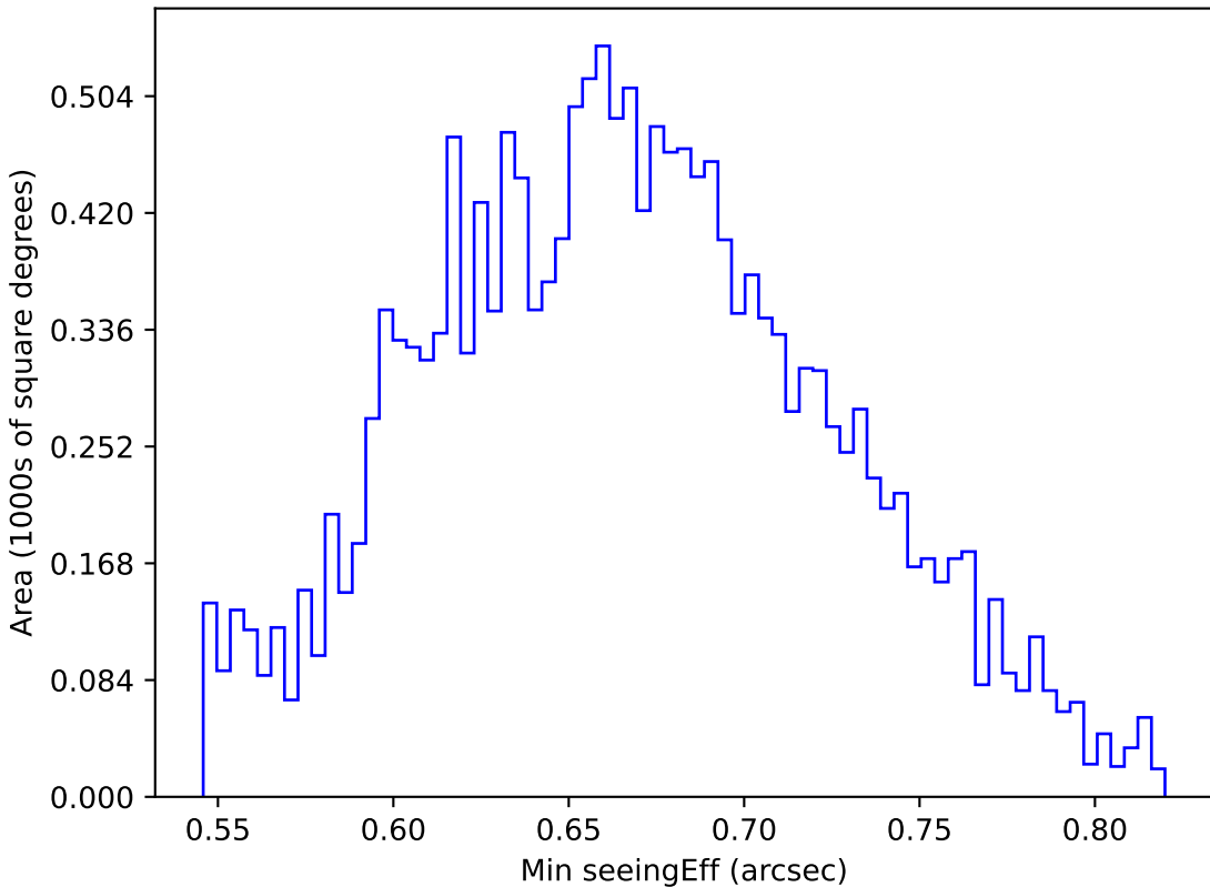
baseline_v2.0_10yrs WFD g band: Min seeingEff
