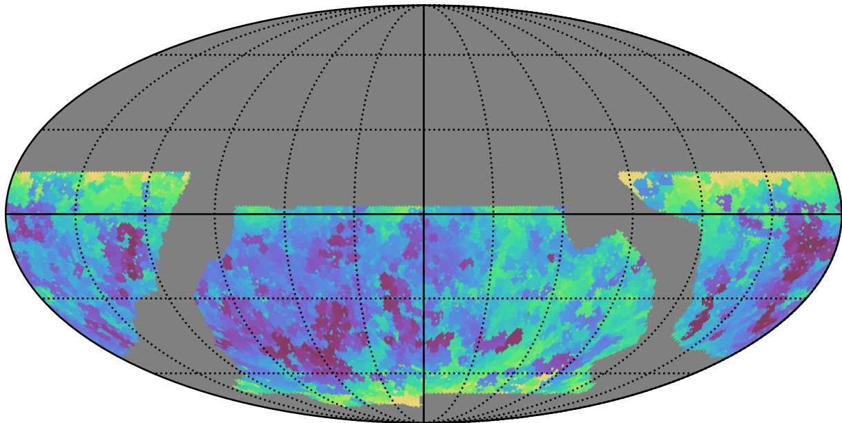
baseline_v2.0_10yrs WFD all bands: Min seeingEff
