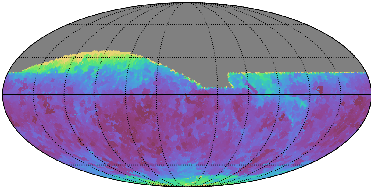
baseline_v2.0_10yrs All sky z band: Min seeingEff
