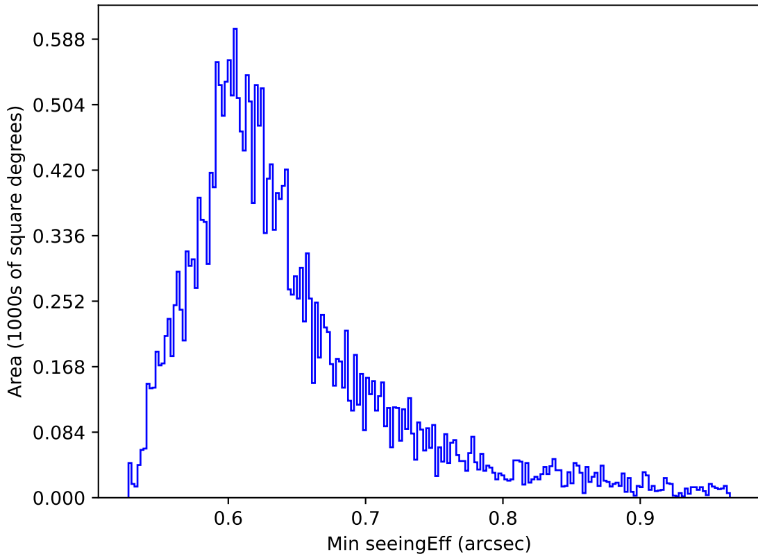
baseline_v2.0_10yrs All sky z band: Min seeingEff
