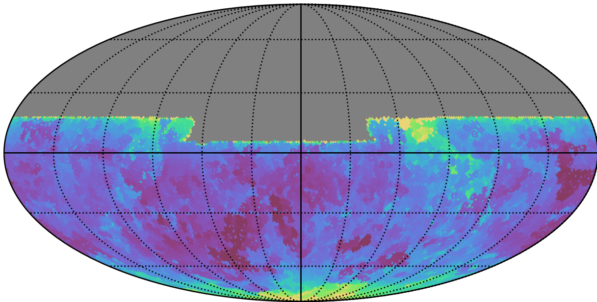
baseline_v2.0_10yrs All sky y band: Min seeingEff
