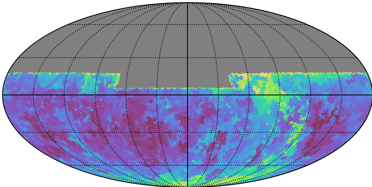
baseline_v2.0_10yrs All sky u band: Min seeingEff
