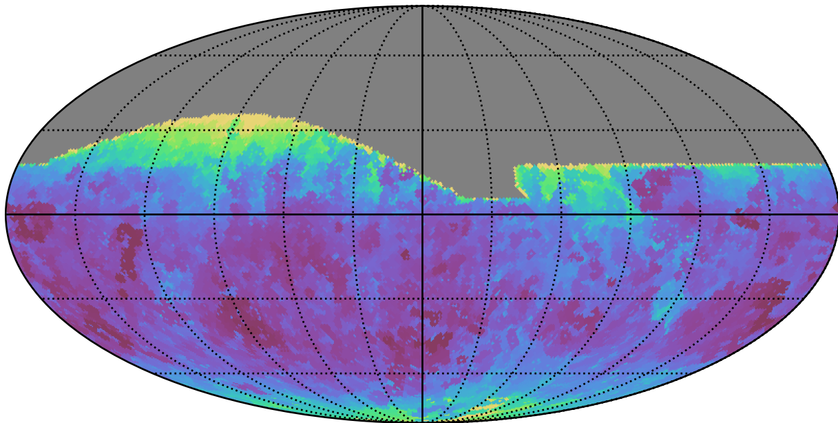
baseline_v2.0_10yrs All sky r band: Min seeingEff
