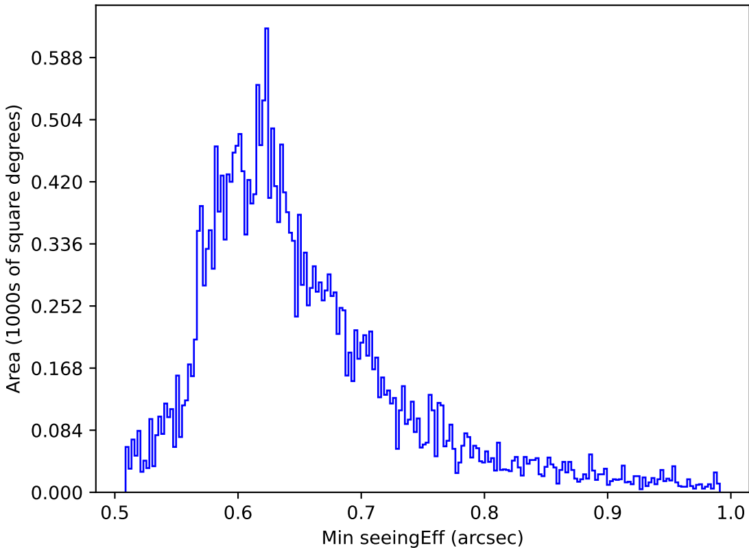
baseline_v2.0_10yrs All sky r band: Min seeingEff
