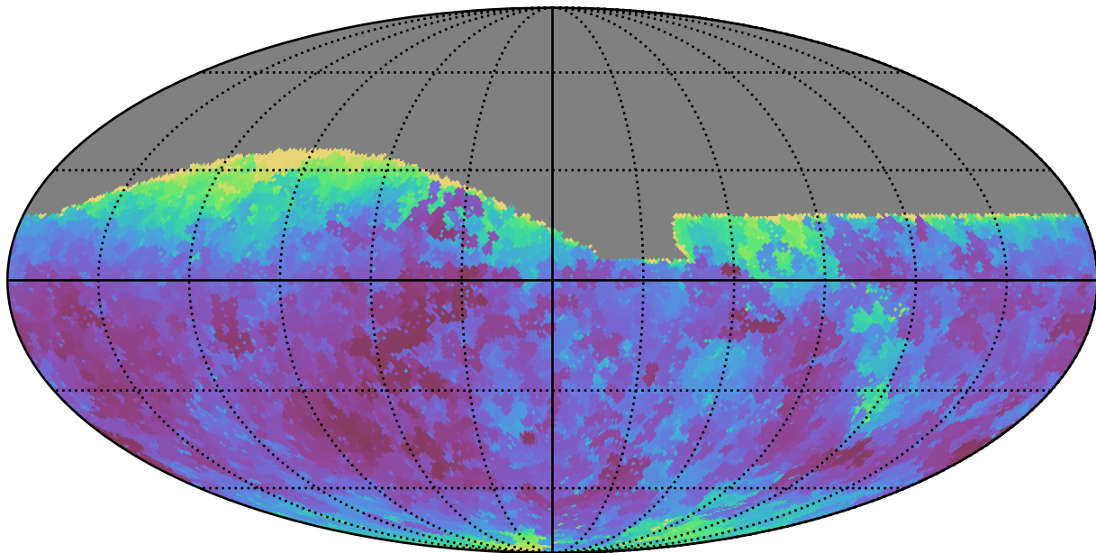
baseline_v2.0_10yrs All sky g band: Min seeingEff
