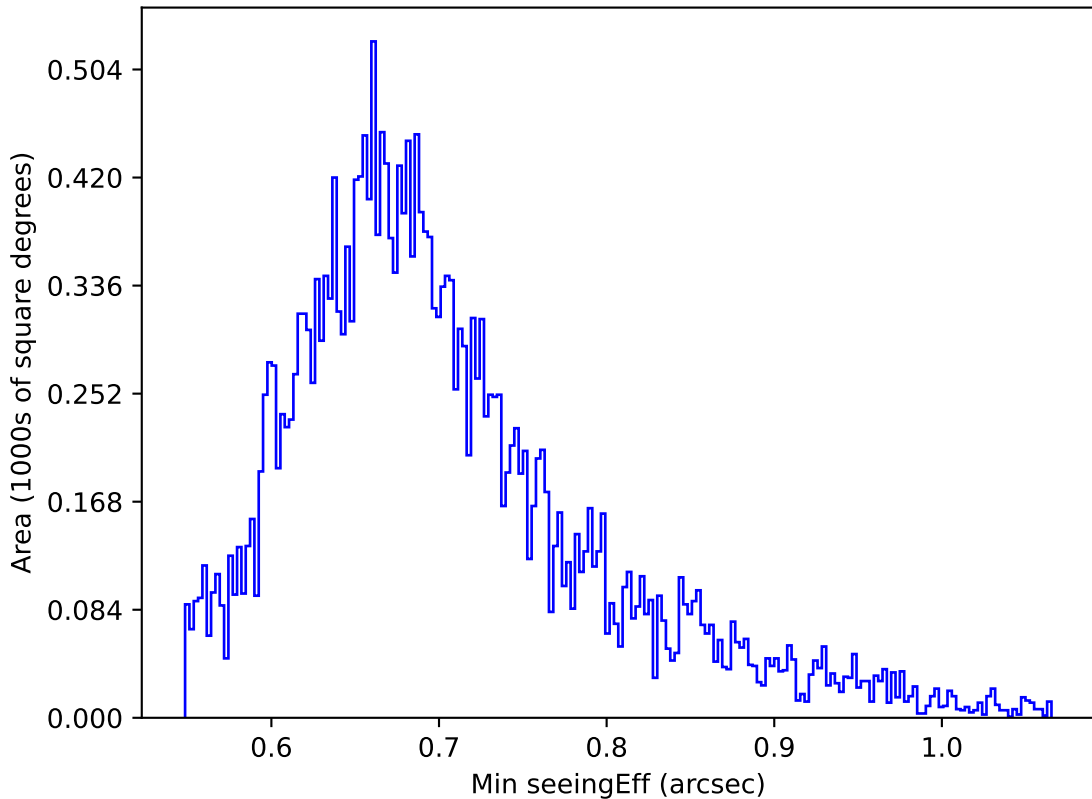
baseline_v2.0_10yrs All sky g band: Min seeingEff
