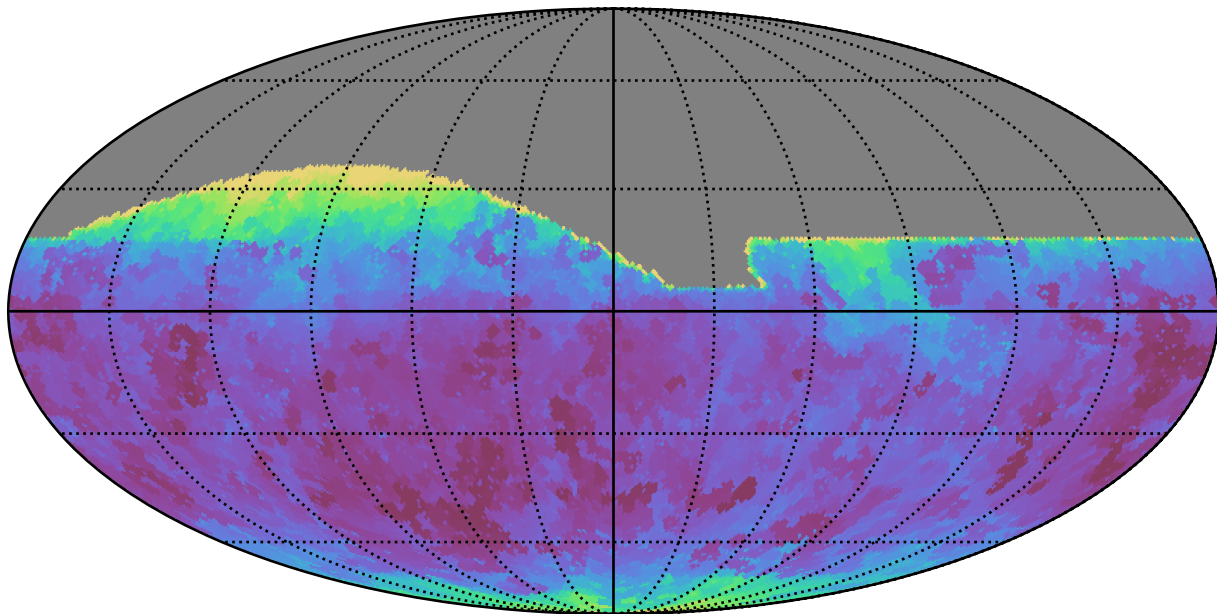
baseline_v2.0_10yrs All sky all bands: Min seeingEff
