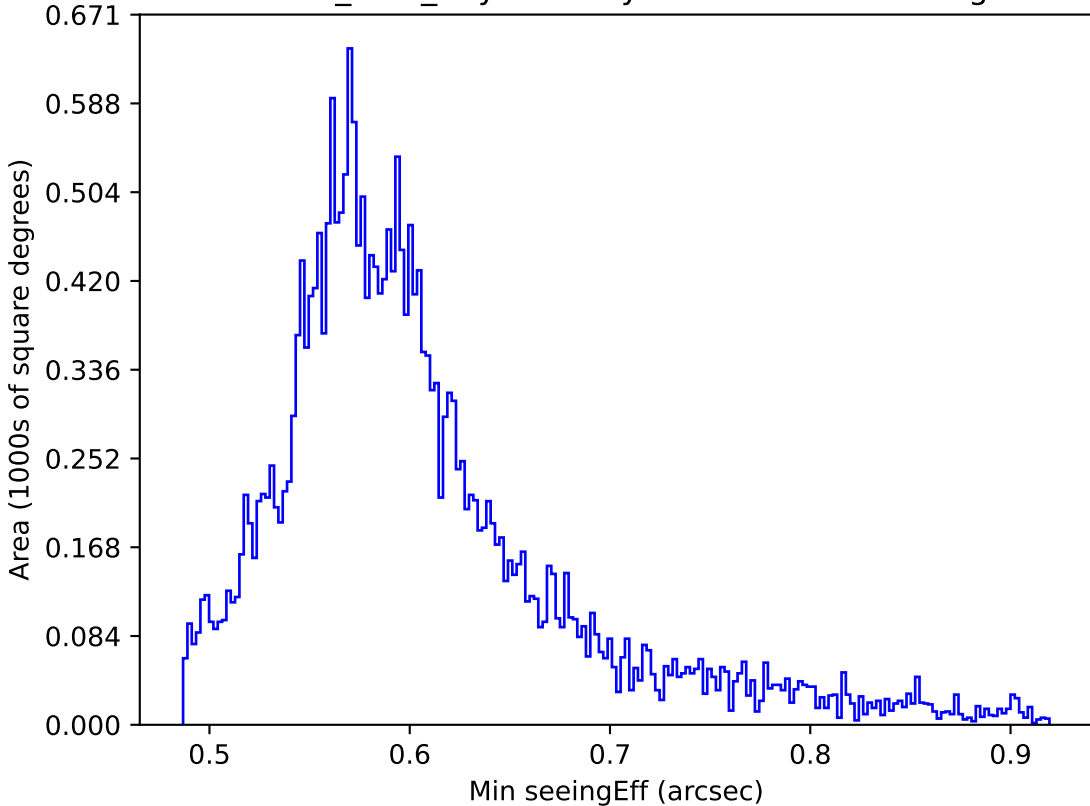
baseline_v2.0_10yrs All sky all bands: Min seeingEff
