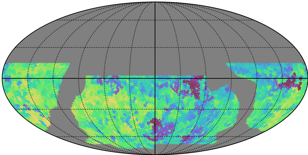
baseline_v2.0_10yrs WFD z band: Min saturation_mag
