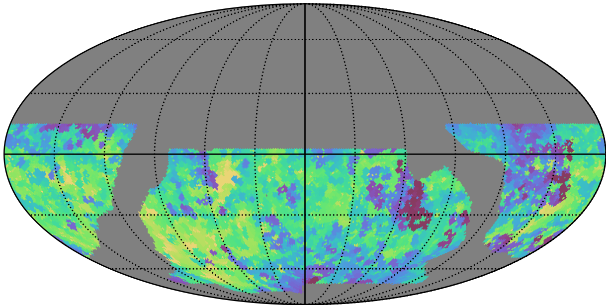
baseline_v2.0_10yrs WFD u band: Min saturation_mag
