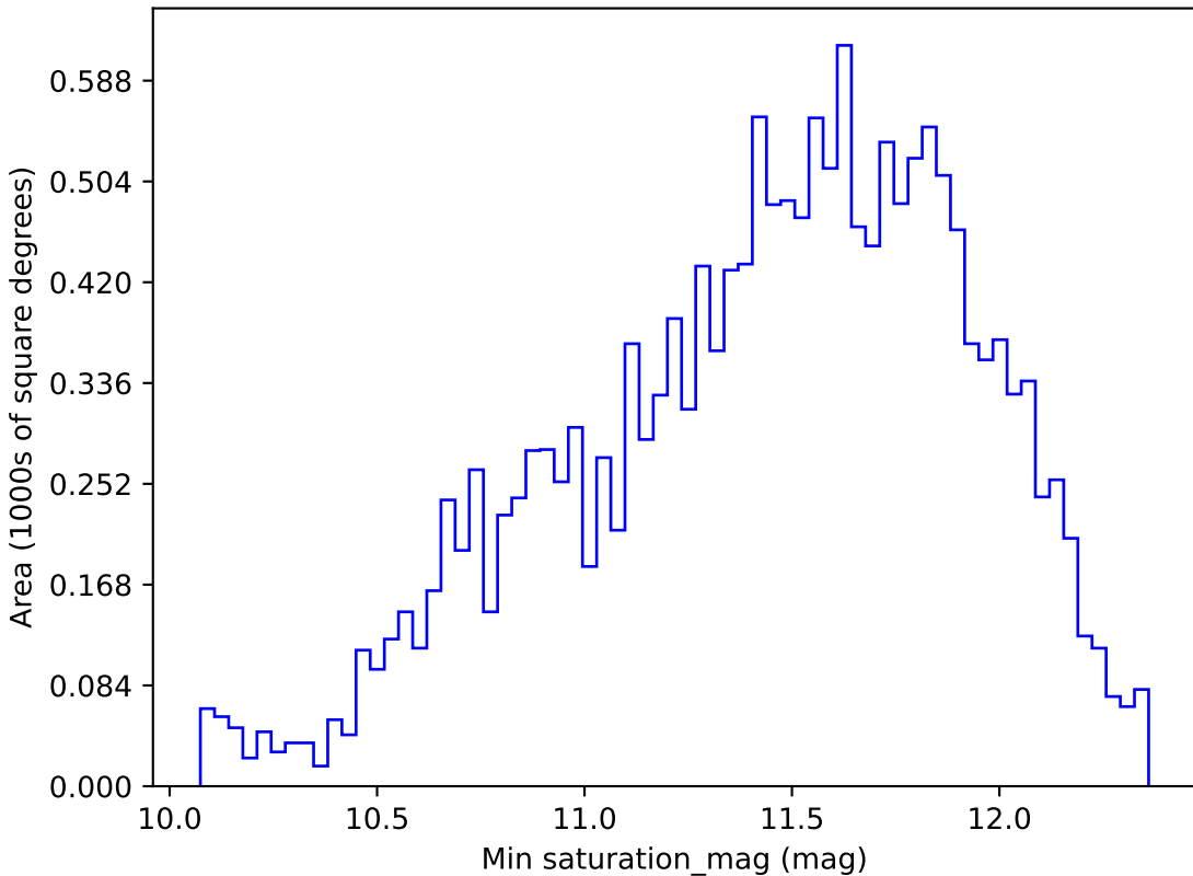
baseline_v2.0_10yrs WFD u band: Min saturation_mag
