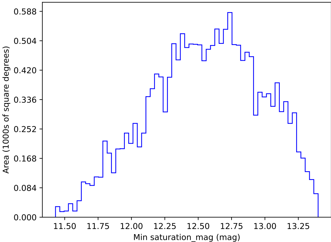
baseline_v2.0_10yrs WFD r band: Min saturation_mag
