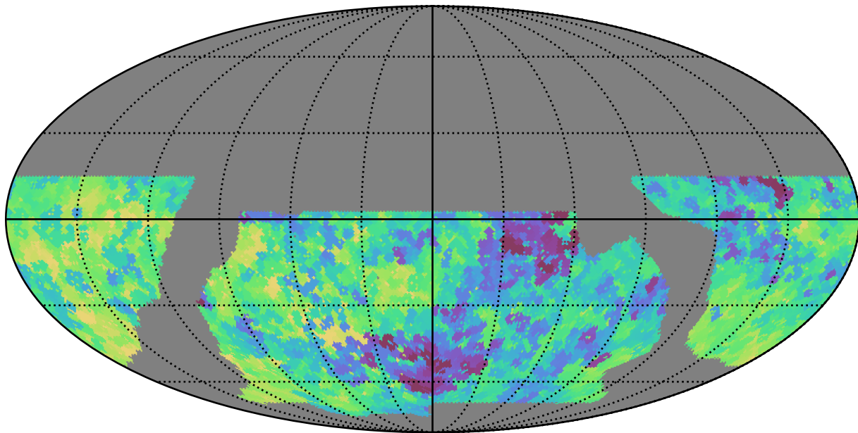
baseline_v2.0_10yrs WFD i band: Min saturation_mag
