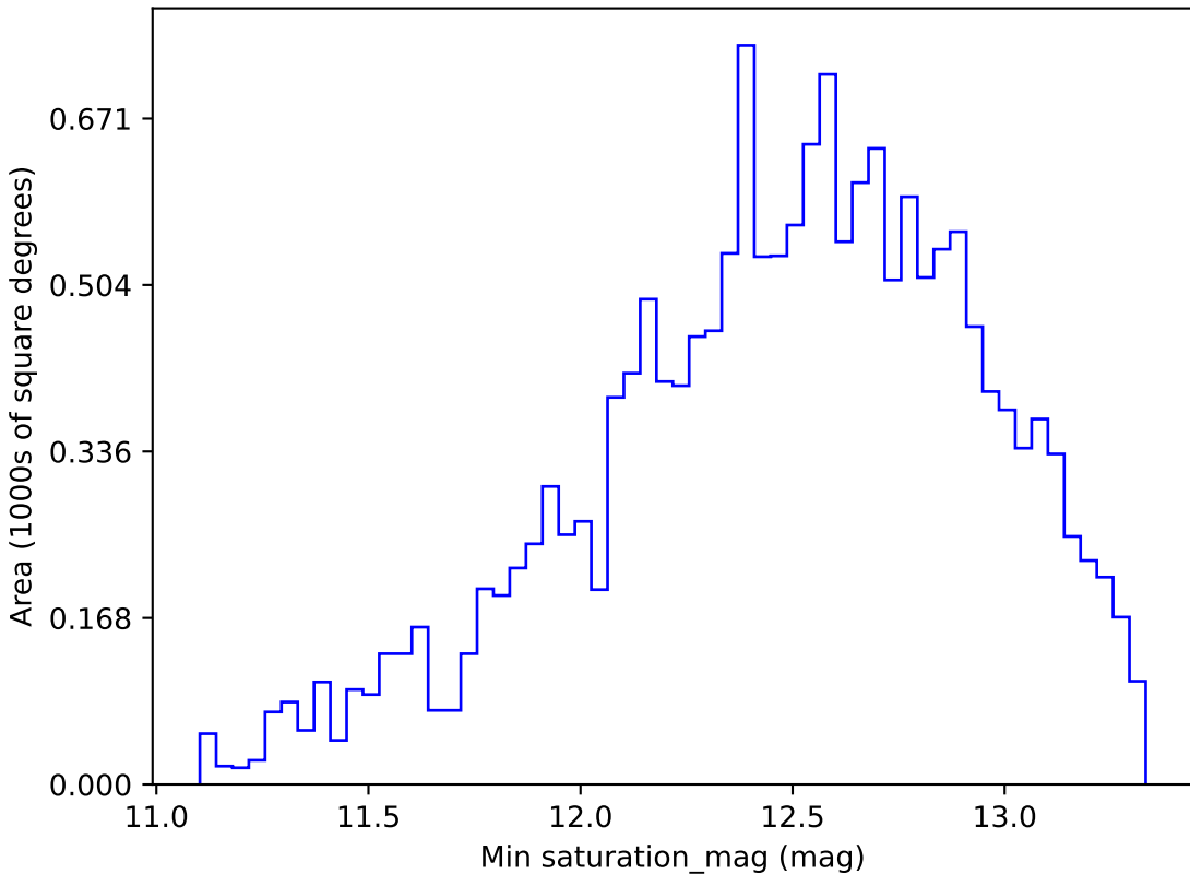
baseline_v2.0_10yrs WFD i band: Min saturation_mag
