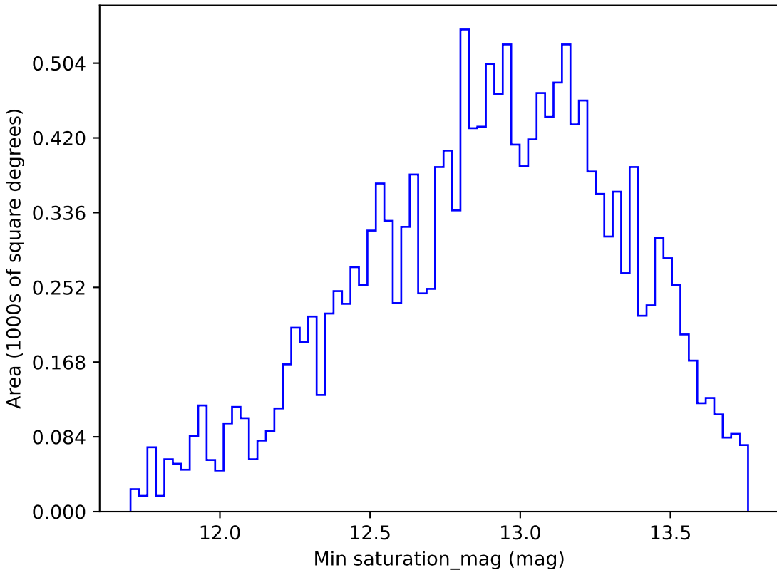
baseline_v2.0_10yrs WFD g band: Min saturation_mag
