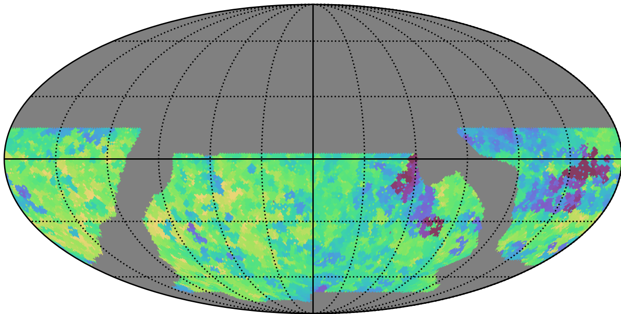
baseline_v2.0_10yrs WFD all bands: Min saturation_mag
