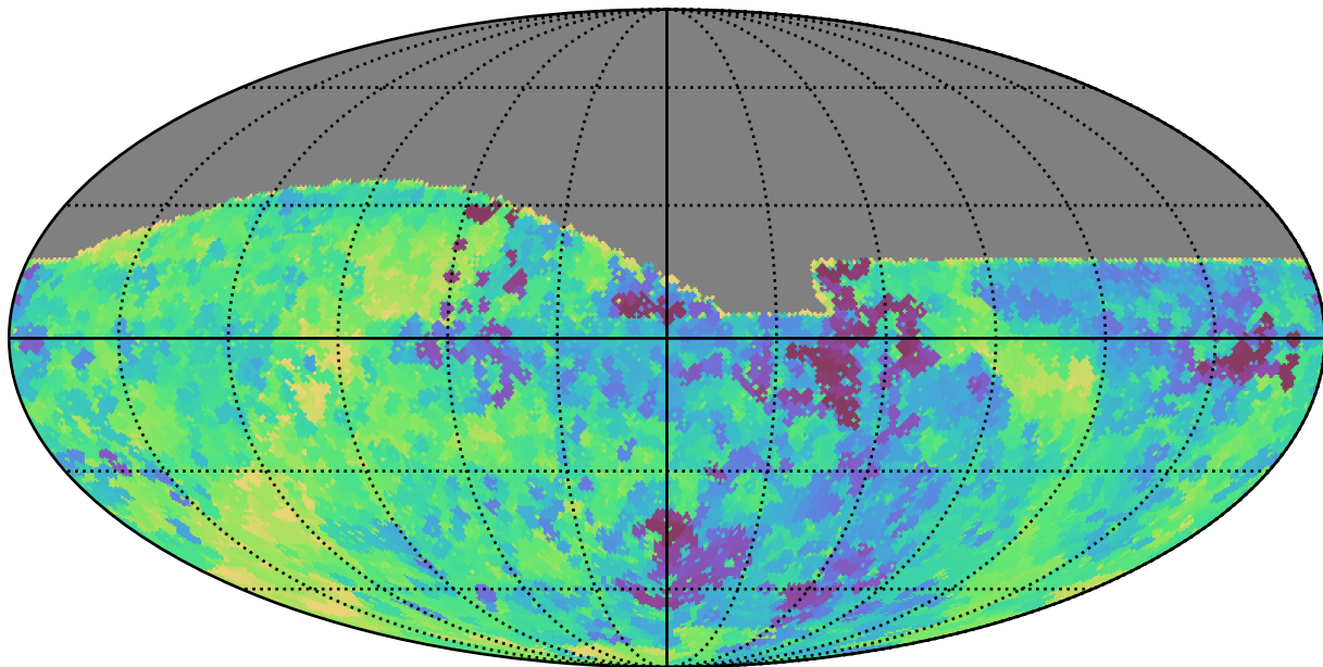
baseline_v2.0_10yrs All sky z band: Min saturation_mag
