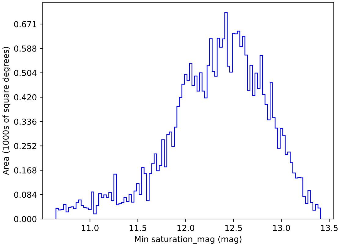
baseline_v2.0_10yrs All sky z band: Min saturation_mag
