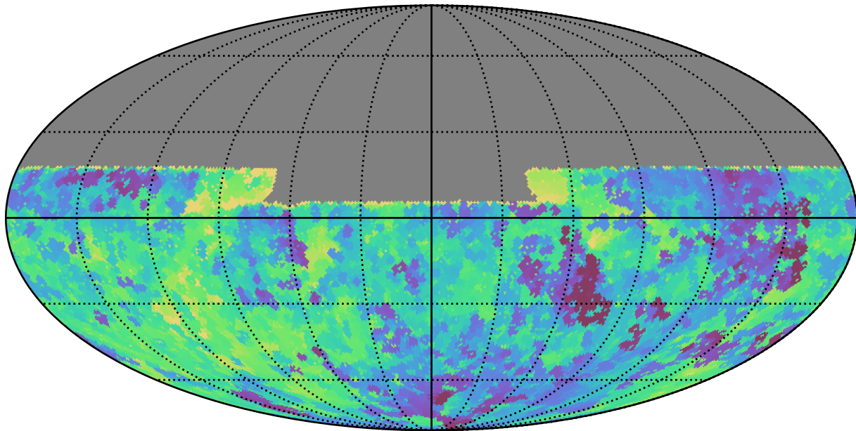
baseline_v2.0_10yrs All sky u band: Min saturation_mag
