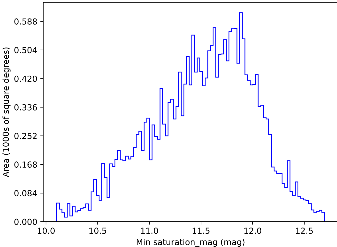
baseline_v2.0_10yrs All sky u band: Min saturation_mag
