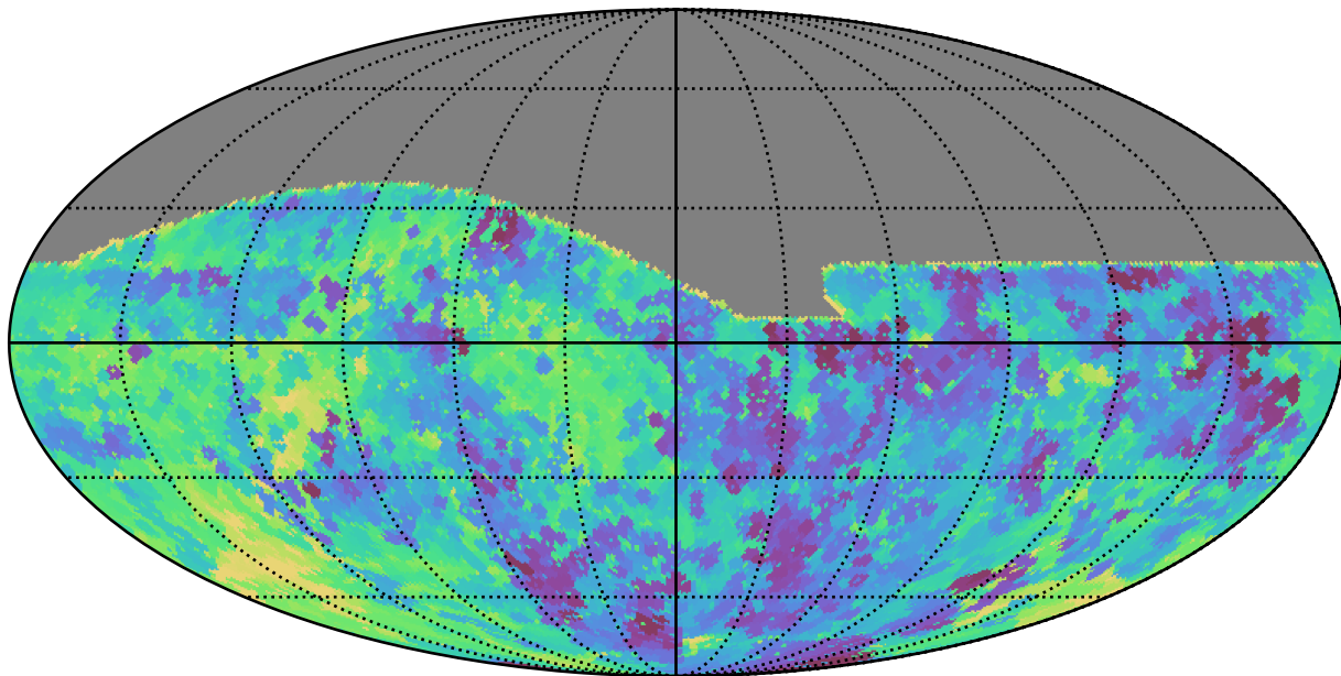
baseline_v2.0_10yrs All sky r band: Min saturation_mag
