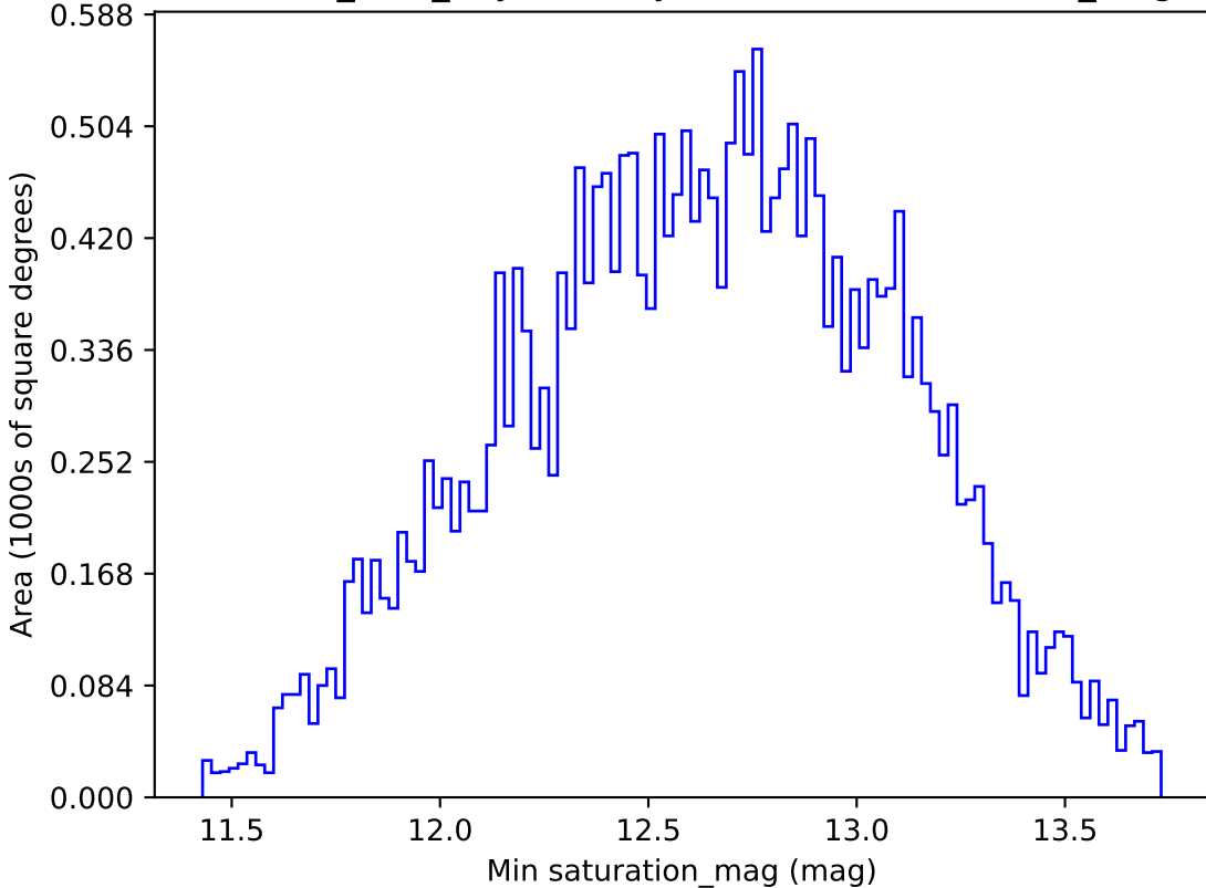
baseline_v2.0_10yrs All sky r band: Min saturation_mag
