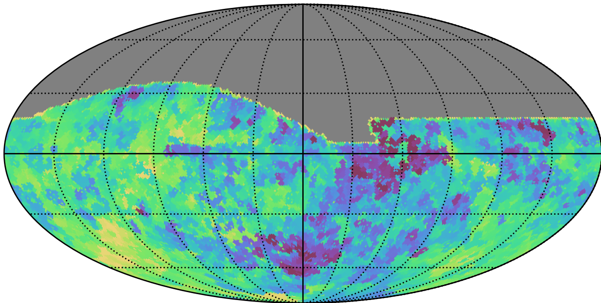
baseline_v2.0_10yrs All sky i band: Min saturation_mag
