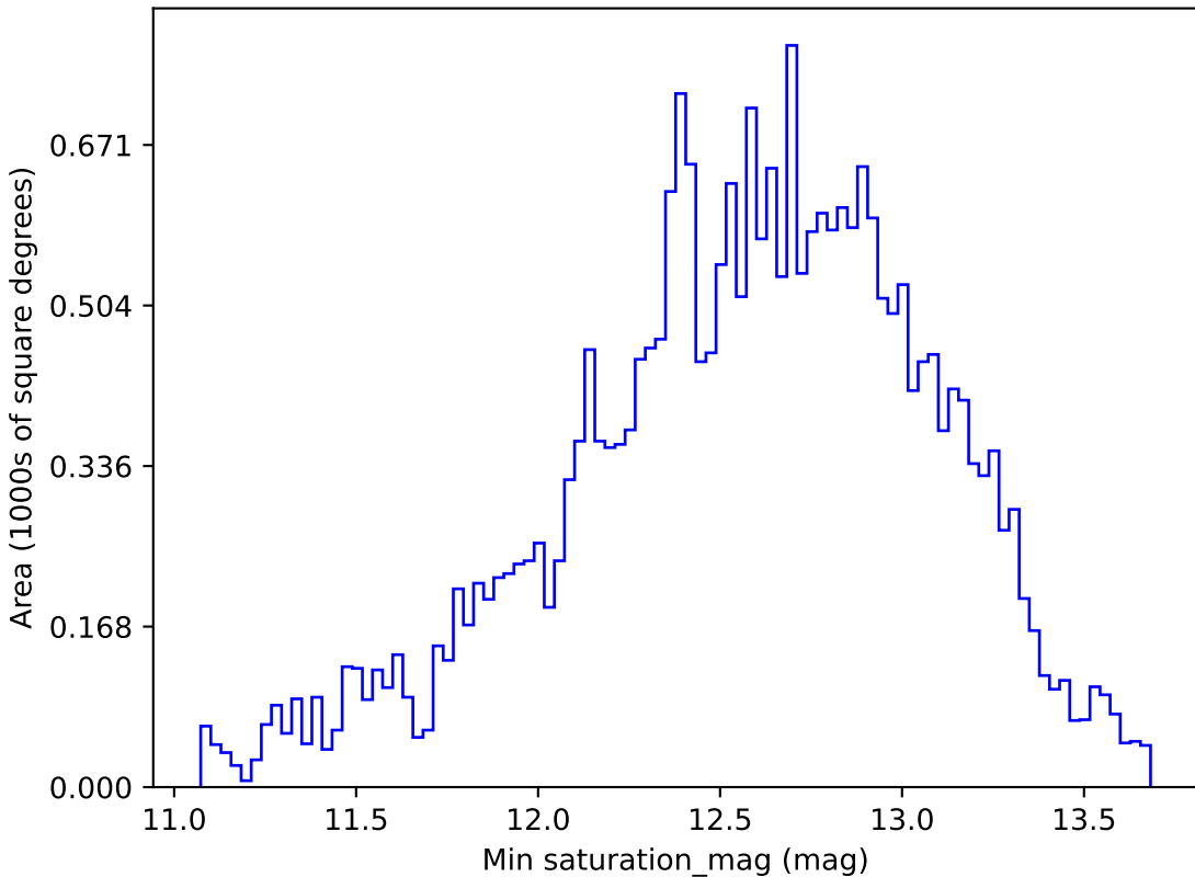
baseline_v2.0_10yrs All sky i band: Min saturation_mag
