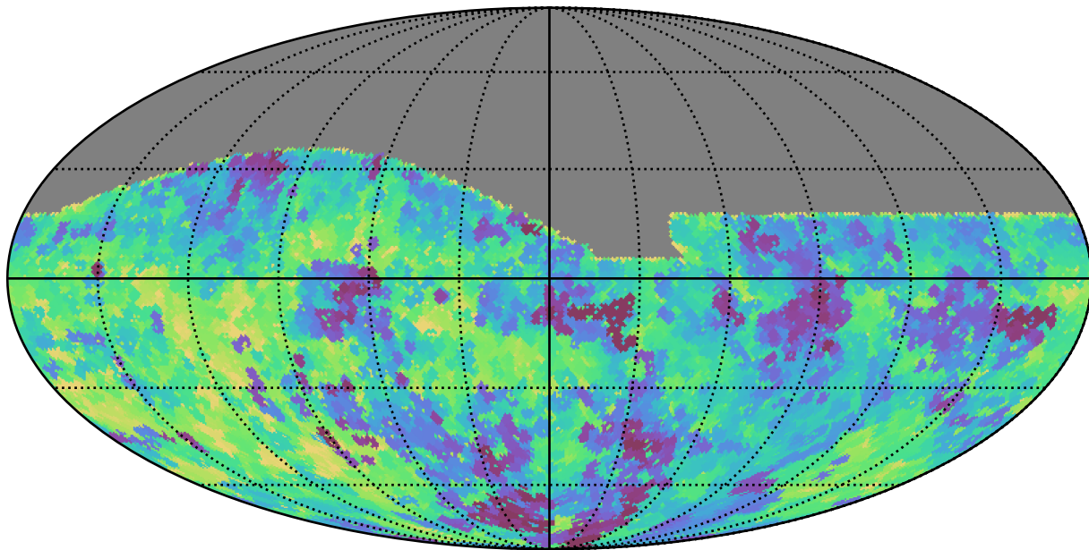
baseline_v2.0_10yrs All sky g band: Min saturation_mag
