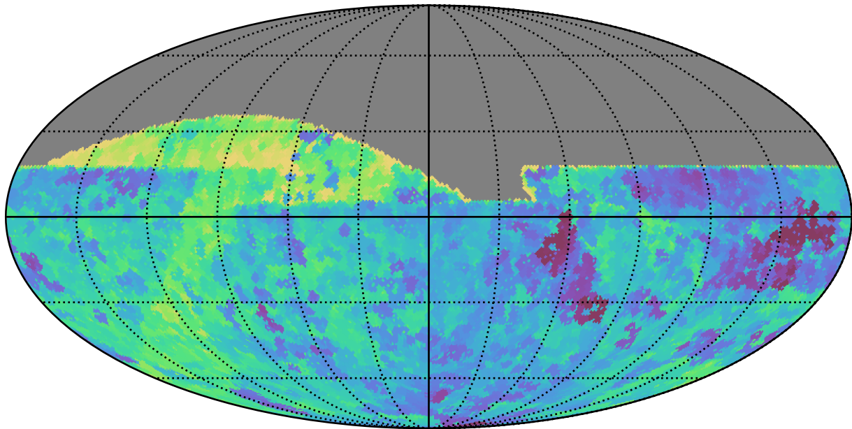
baseline_v2.0_10yrs All sky all bands: Min saturation_mag
