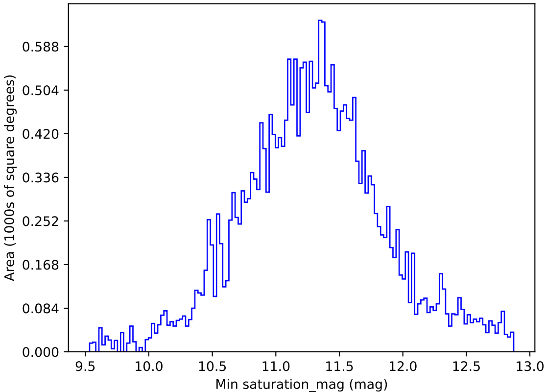
baseline_v2.0_10yrs All sky all bands: Min saturation_mag
