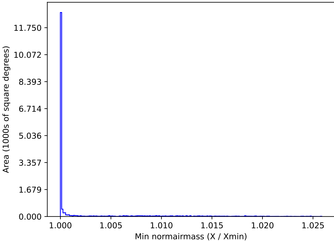
baseline_v2.0_10yrs WFD z band: Min normairmass
