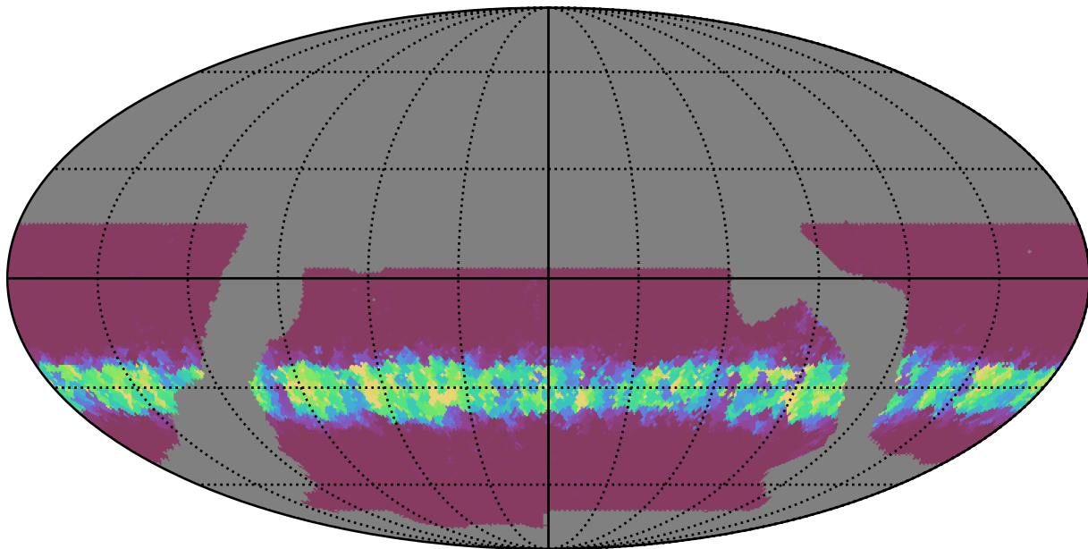
baseline_v2.0_10yrs WFD u band: Min normairmass
