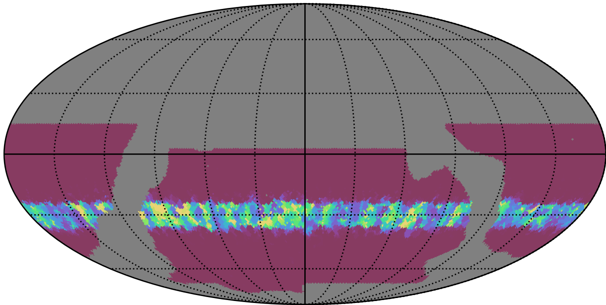
baseline_v2.0_10yrs WFD r band: Min normairmass
