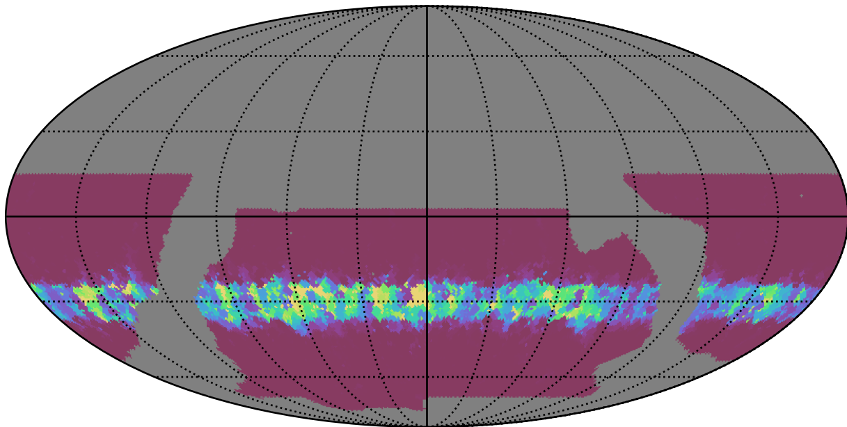
baseline_v2.0_10yrs WFD g band: Min normairmass
