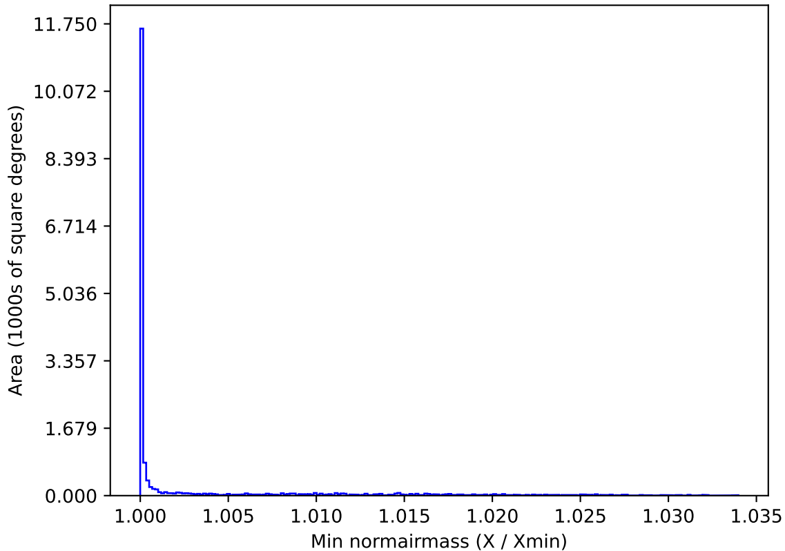
baseline_v2.0_10yrs WFD g band: Min normairmass
