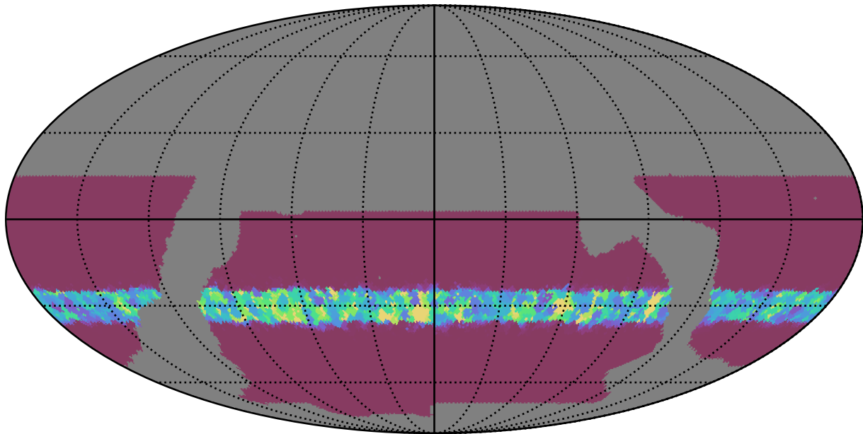
baseline_v2.0_10yrs WFD all bands: Min normairmass
