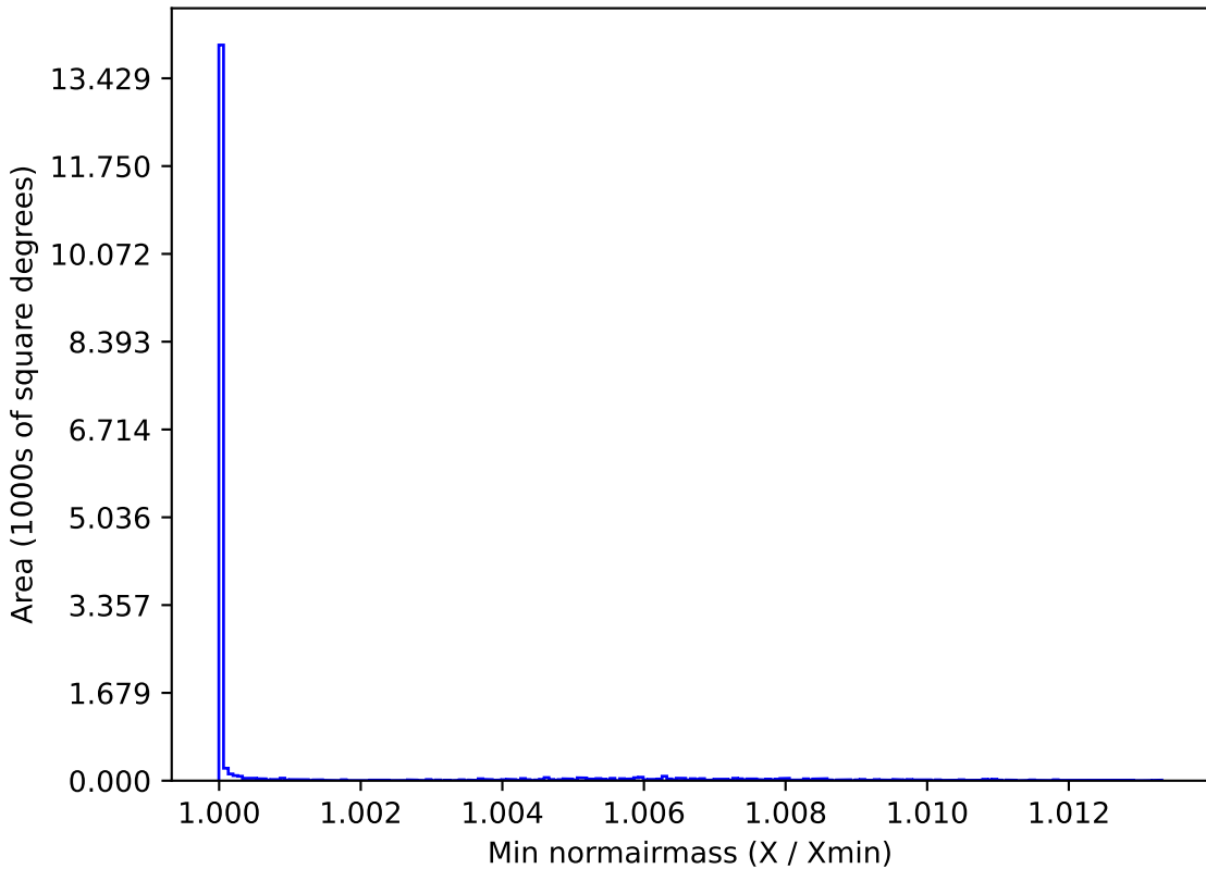
baseline_v2.0_10yrs WFD all bands: Min normairmass
